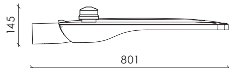
Dimensions with NEMA socket
