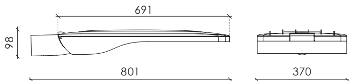
Dimensions with 60 mm console
